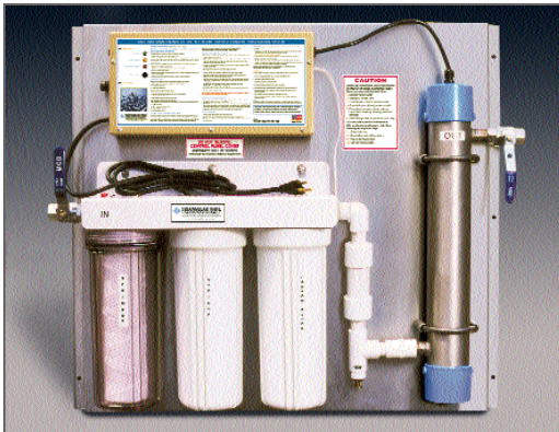
TWT-MD-1002 Triangular Wave Technologies Fluid Management System. System consists of a Deposit Controller TWT-5C8-472 • TWT Reaction Chamber • UV-250 Disinfection System and TWT-MUC Filtration System Specifications: Factory assembled and mounted 24" H x 26.5" W x 8" D • Weight 30 lbs.
