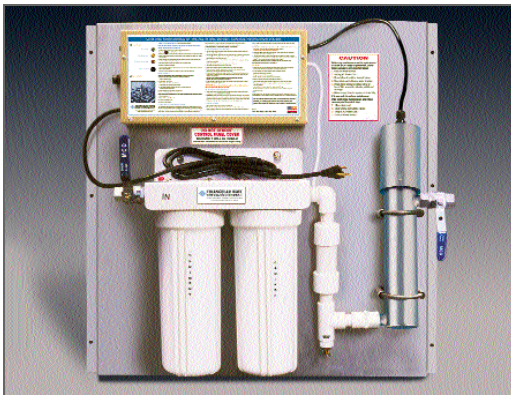
TWT-MD-1001 Triangular Wave Technologies Water Fluid Management System. System consists of a Deposit Controller TWT-5C8-471 • TWT Reaction Chamber • UV-4 Disinfection System and TWT-MUC Filtration System Specifications: Factory assembled and mounted 24" H x 22" W x 8" D • Weight 25 lbs.
